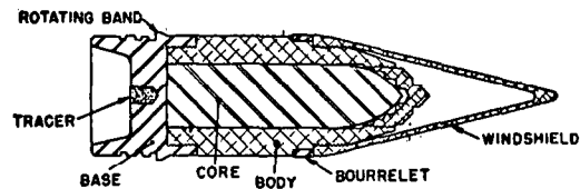
TYPICAL H.V.A.P. SHOT
